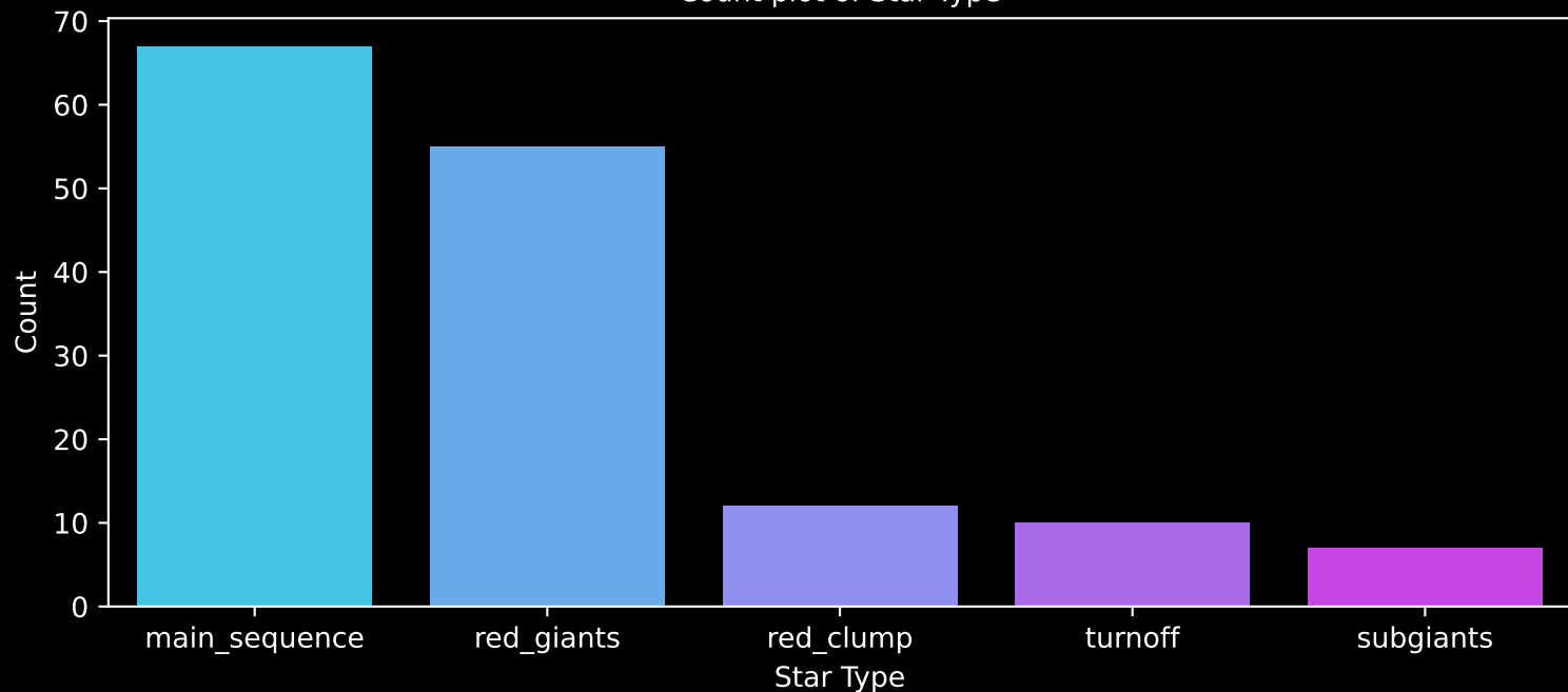
APOGEE DR17 Field: [K2_C6_316+48_btx] Count plot of Star Type
