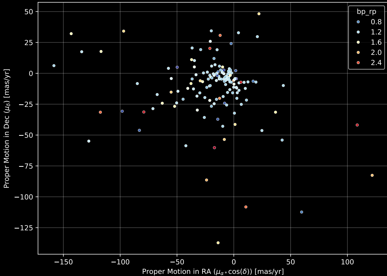
APOGEE DR17 Field: [K2_C6_316+48_btx] Proper Motion Diagram (n= 151)
