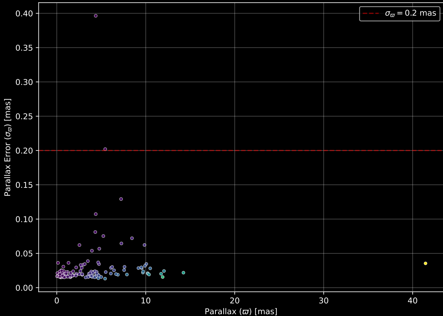
APOGEE DR17 Field: [K2_C6_316+48_btx] Parallax Quality (n= 151)
