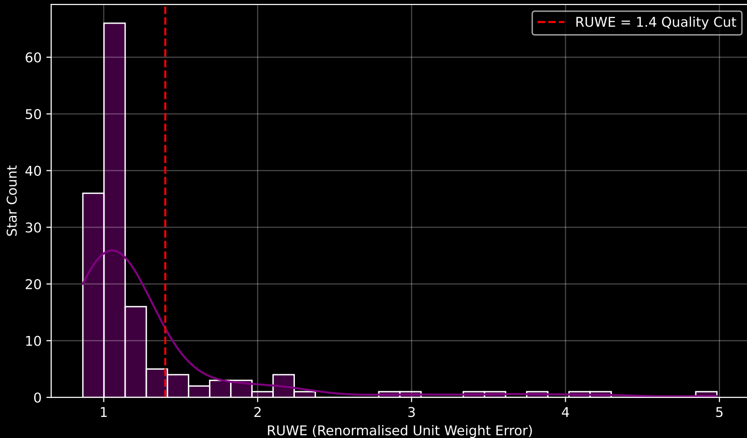
GAPOGEE DR17 Field [K2_C6_316+48_btx] RUWE Distribution (n= 149)
