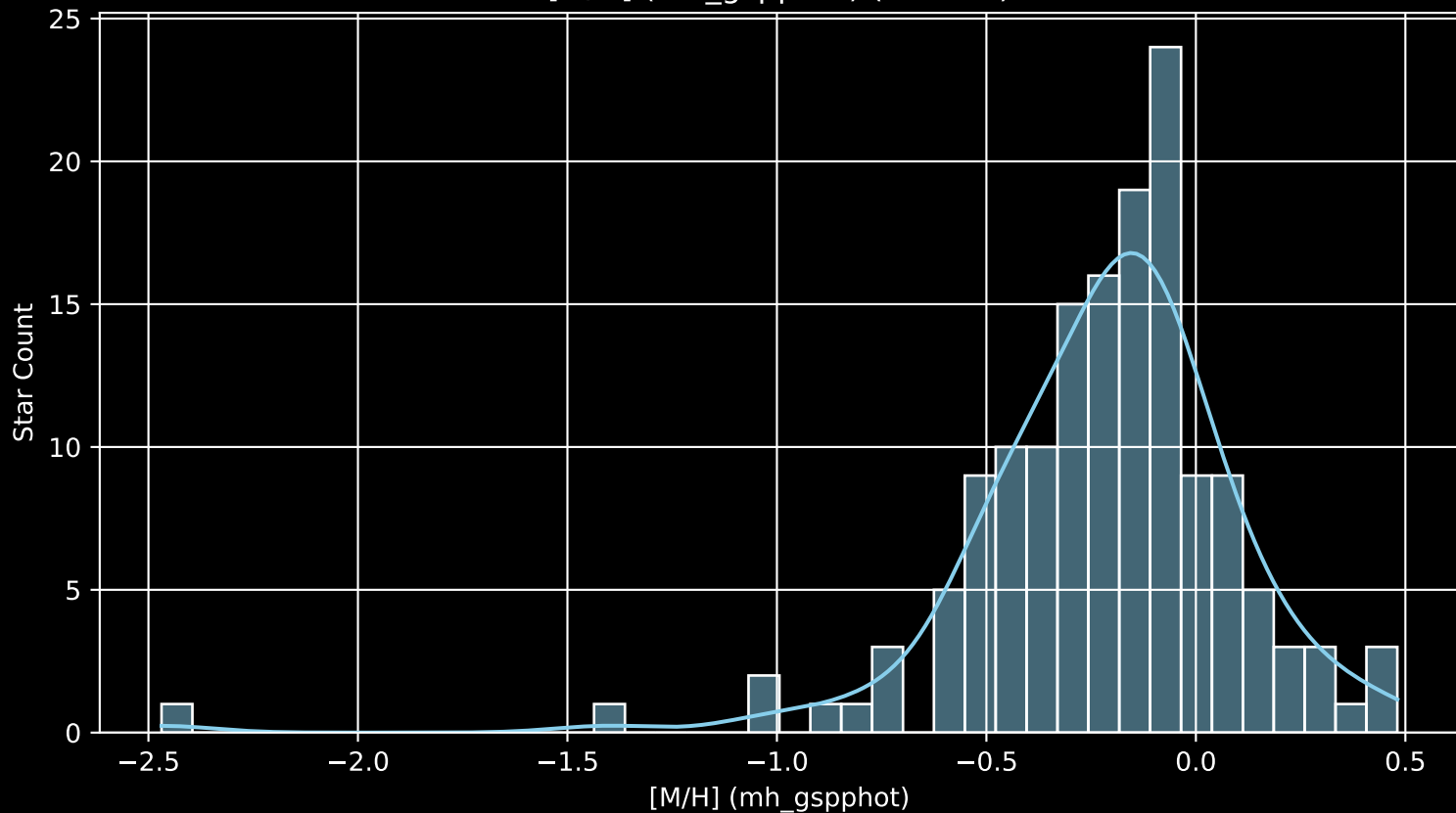
APOGEE DR17 Field: [K2_C6_316+48_btx [M/H] (mh_gspphot) (n= 150)
